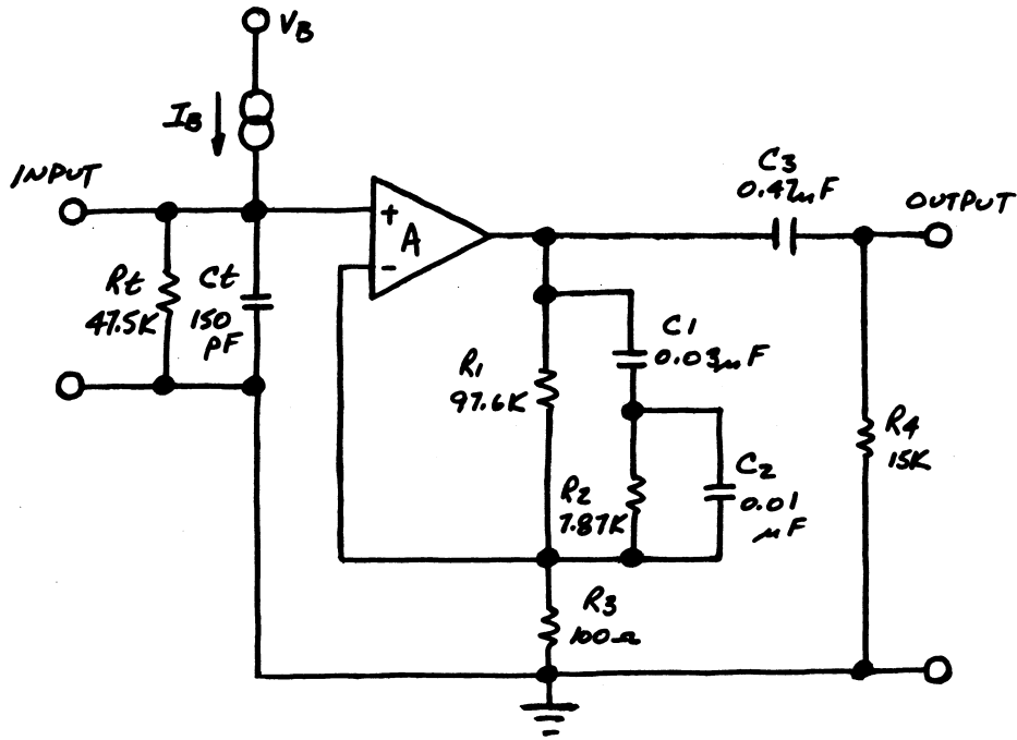
Fig. 1: FEEDBACK EQUALIZED PHONO PREAMP
