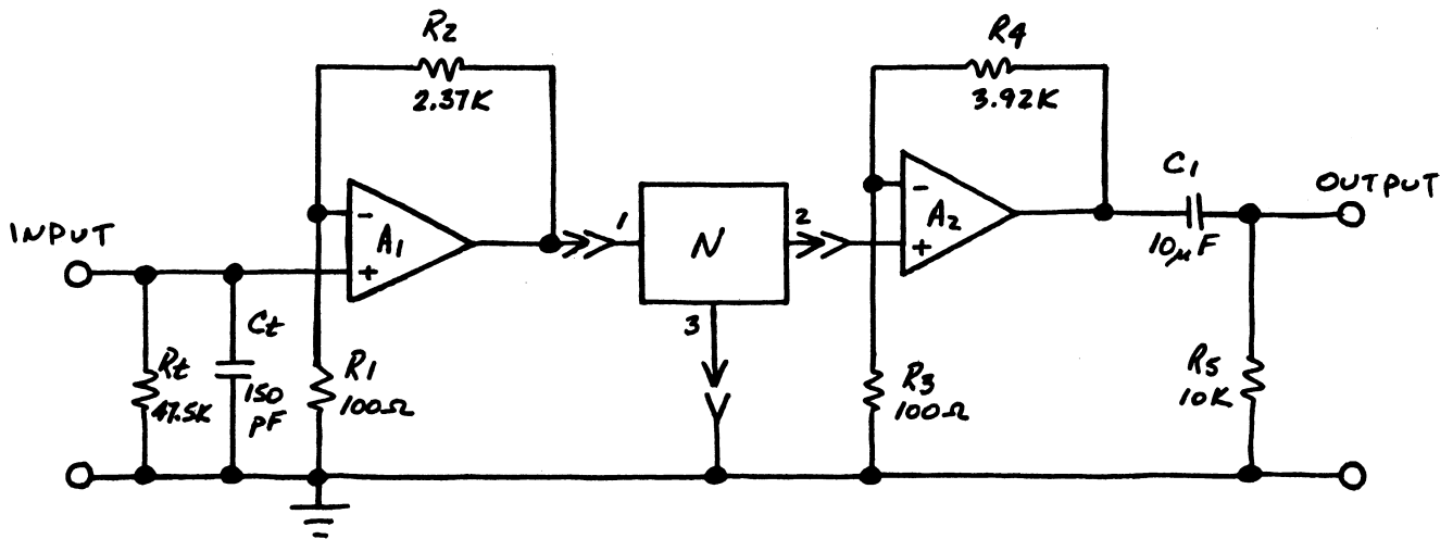
Fig. 2: PASSIVELY EQUALIZED PHONO PREAMP
