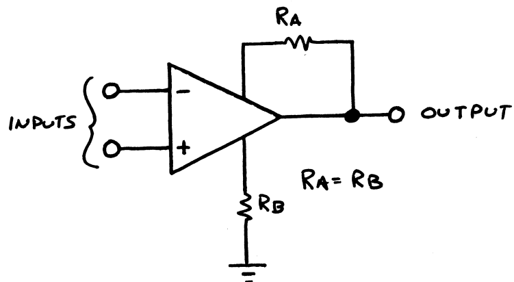
Fig. 4: TRANSCONDUCTANCE-MODE OPERATION OF OPAMP DEVICE
